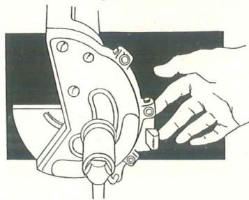
On our fence, once the stops at 45 and 90 degrees have been set, there is never again any necessity to use the square or bevel. A flip of the finger takes the stop out of the way for tilting.
